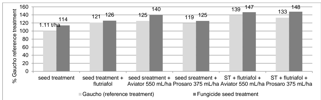
Figure 1. %Yield relative to nil fungicide (Gaucho), 1.11 t/ha in Crusher canola, 10/11/16 (180 DAA/ 134 DAC)
